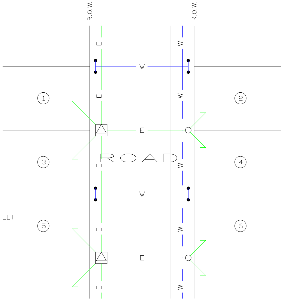
PLAN VIEW
